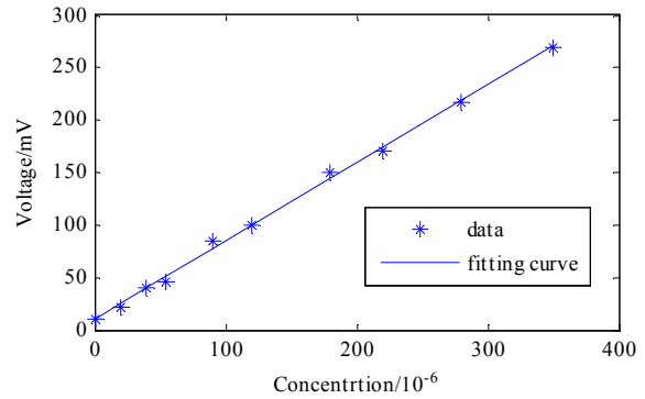
Figure 11. The fitting curve between the SO 2 concentration and the measured voltage value after EMD denoising.
