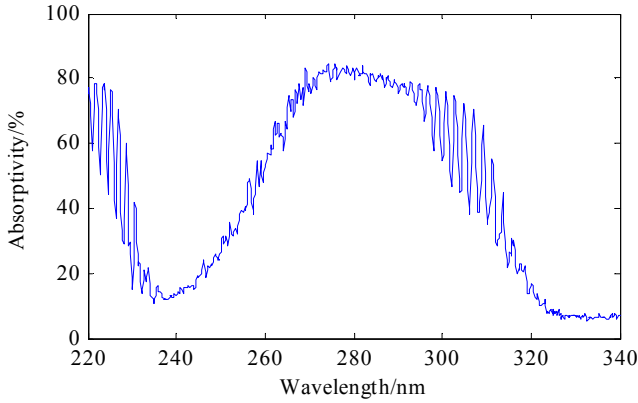
Figure 3. The ultraviolet absorption spectrum of SO 2 .
