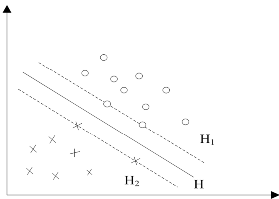
Figure 1. Optimization classify hyperplane under linear condition.
